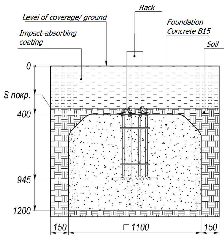
Picture 1 - Concreting scheme of embedded element
