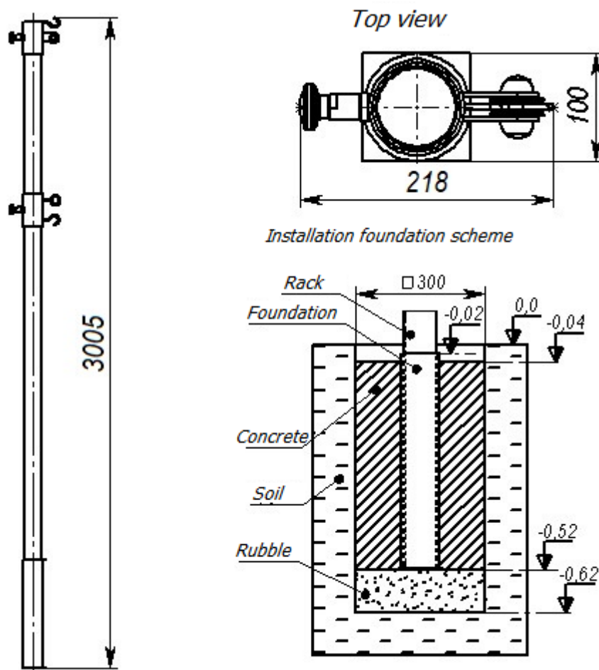
Picture 2 «Product overall dimensions and installation scheme»
