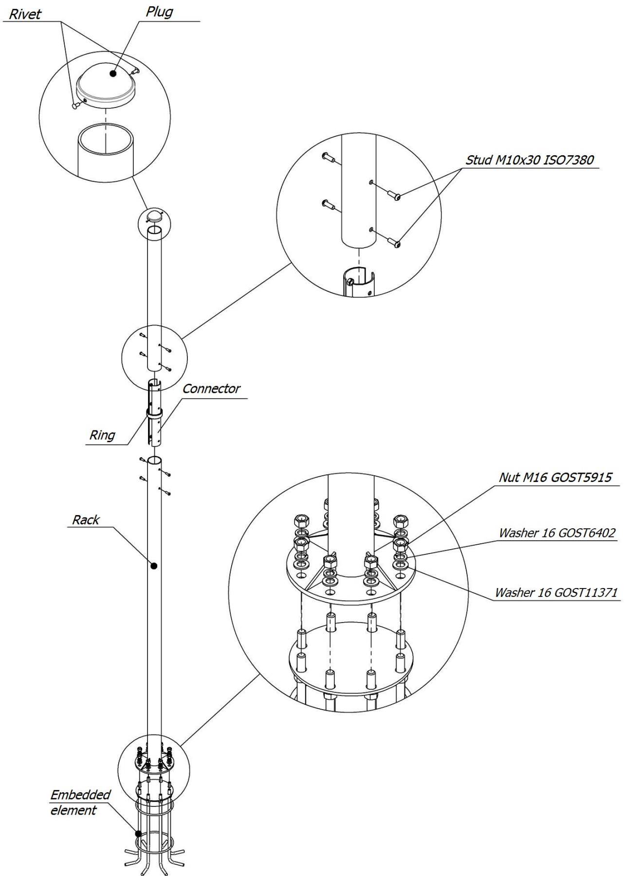
Picture 21 – Assembly scheme of Rack
