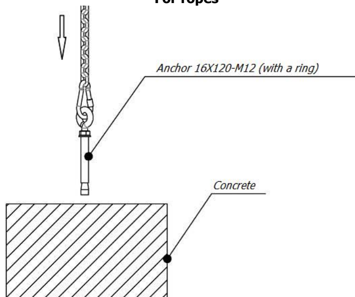
Picture 1.1 – Concreting scheme
