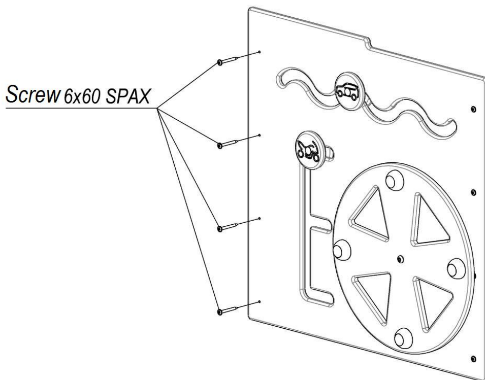
Picture 2 – Fixing panel scheme (Fixing other details is identical)
