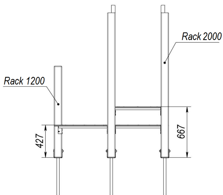
Picture 3 – Rack assembly scheme
