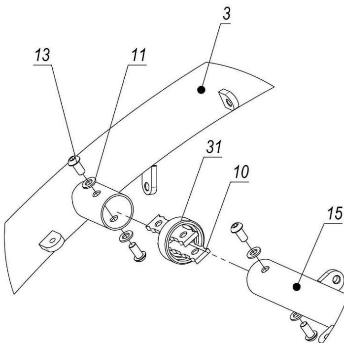
Picture 3 – Rack assembly scheme
