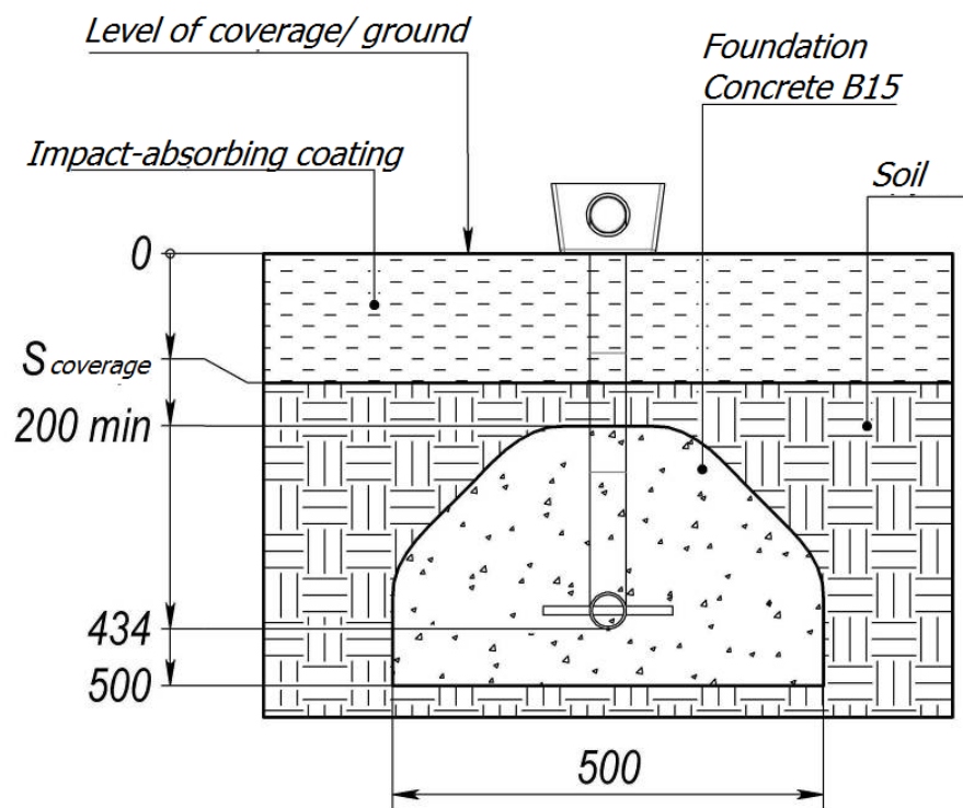
Picture 1 – Concreting schemes
