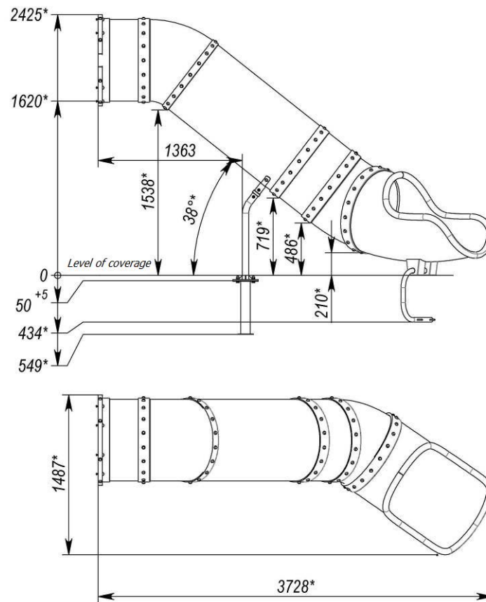
Picture 4 – Overall dimensions
