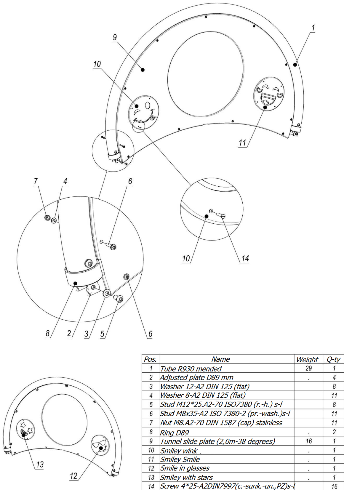
Picture 2 – Tubes and plate assembly scheme
