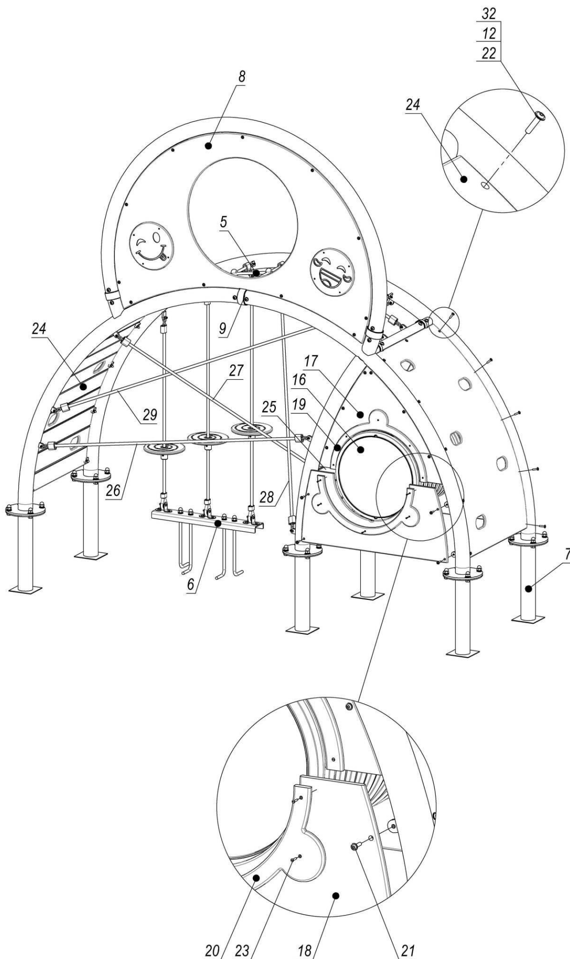
Picture 3.1 – Cord and climb with tunnel fixing schemes (bores in climbs with 4/5 adapters pos.24,25 must be bored at the place of assembling)
