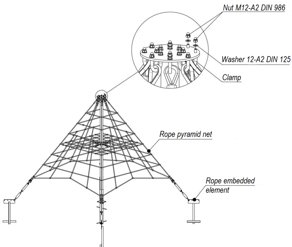
Picture 1 – Rack installation scheme
