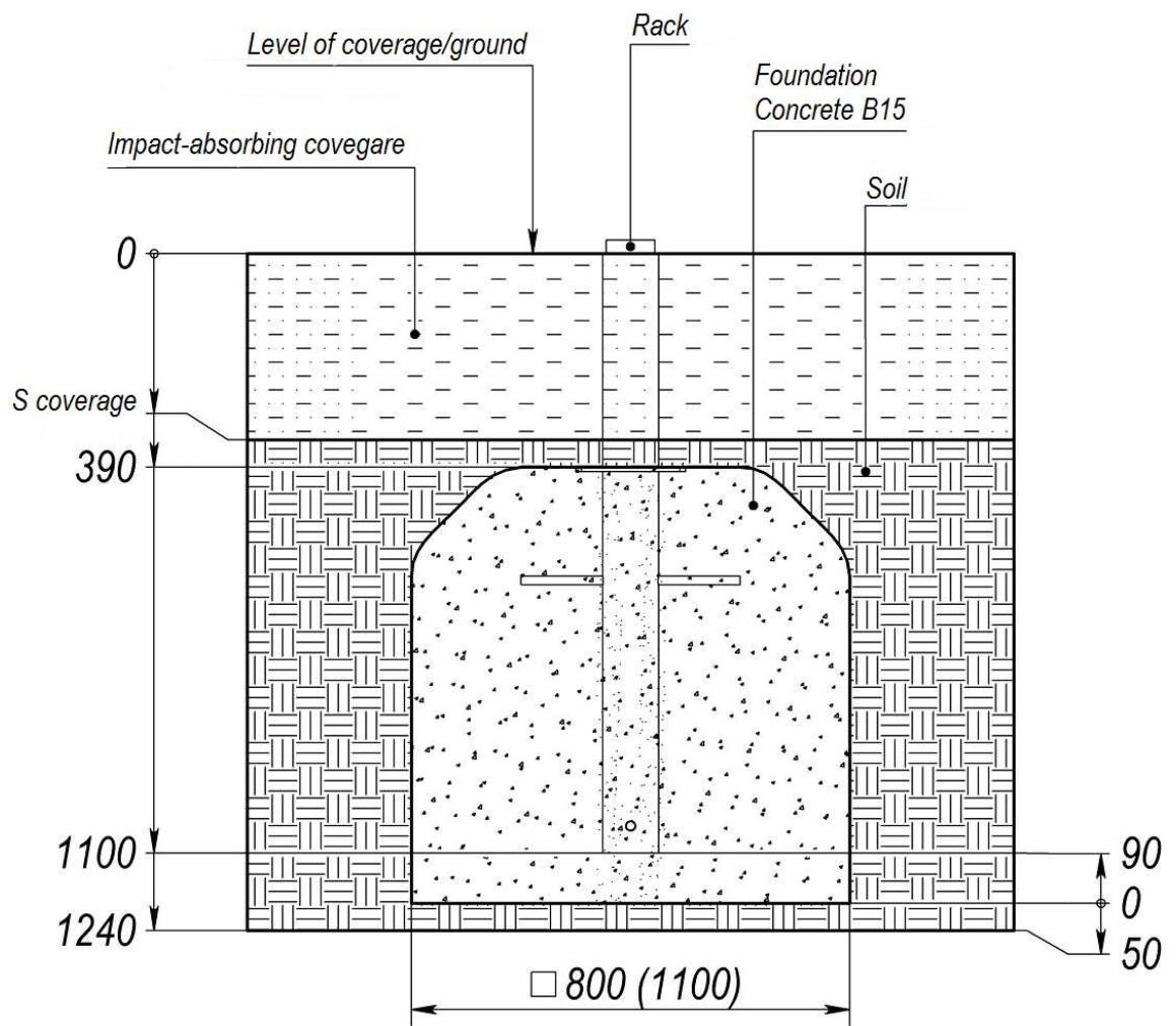
Picture 3 – Concreting scheme of embedded elements
