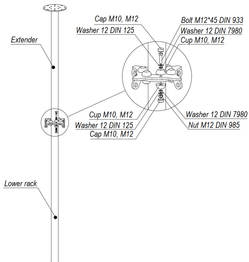
Picture 1 – Rack installation scheme
