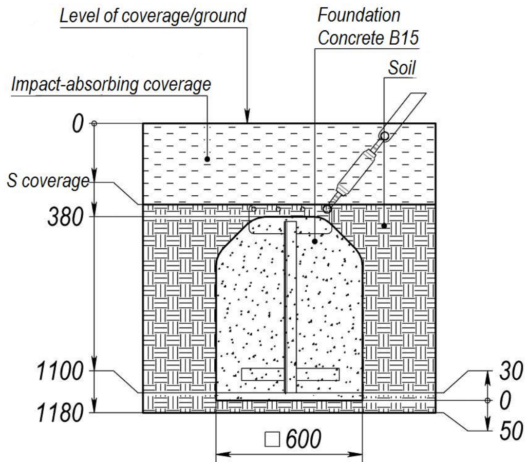
Picture 4 – Concreting scheme of embedded side elements
