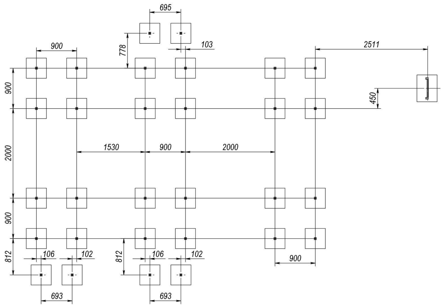
Layout scheme of foundation
