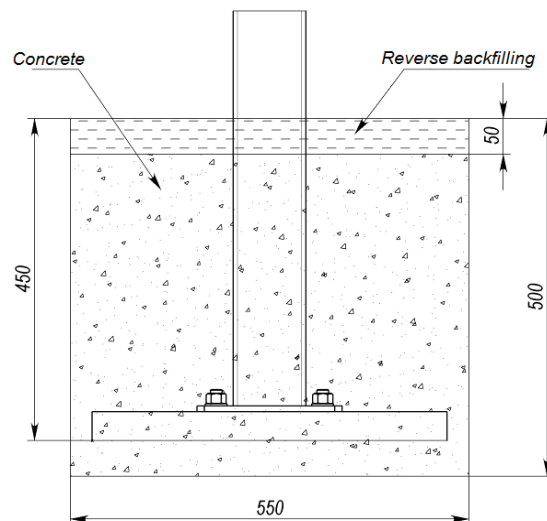
Picture 5 – Scheme of foundation installation
