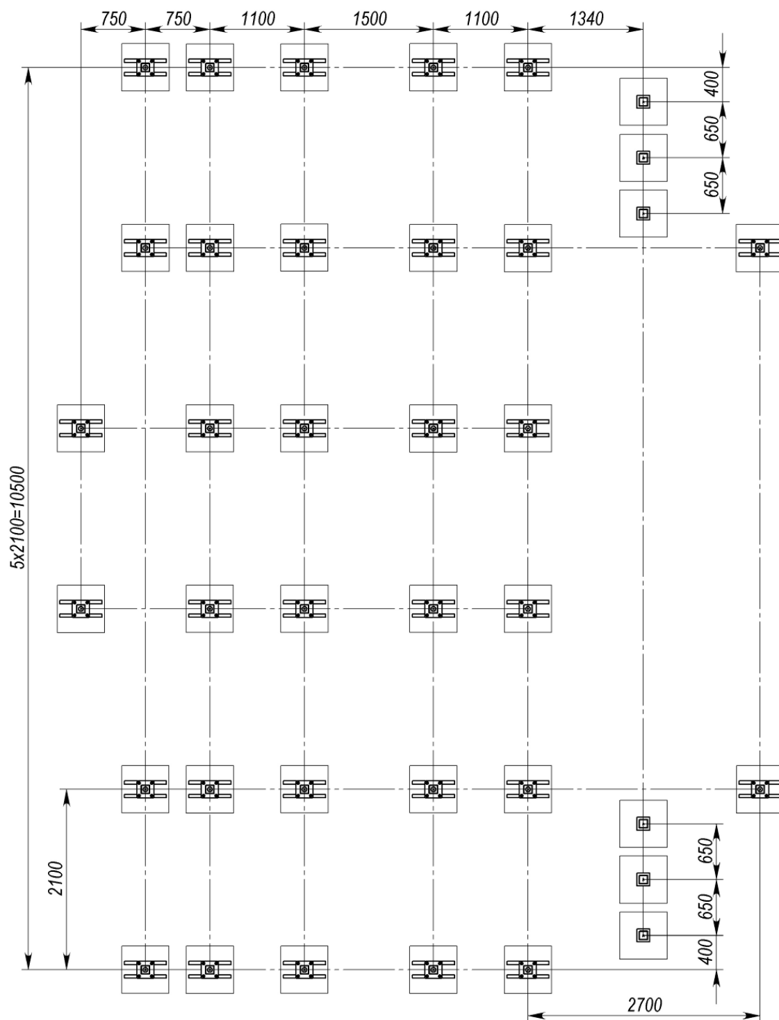
Picture 3 – Concreting zone for UT131
