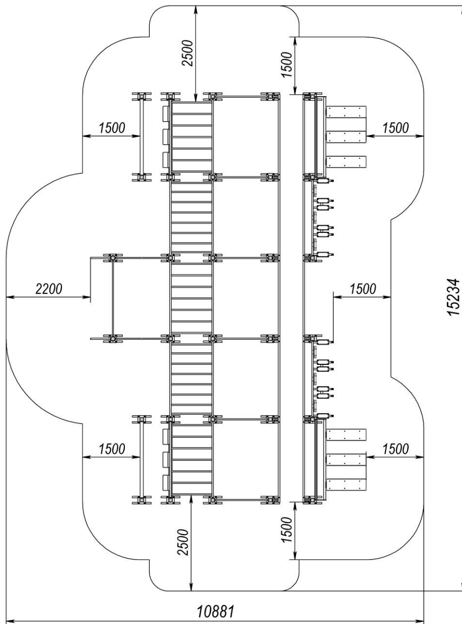
Picture 7 – Safety zone for UT131-584
