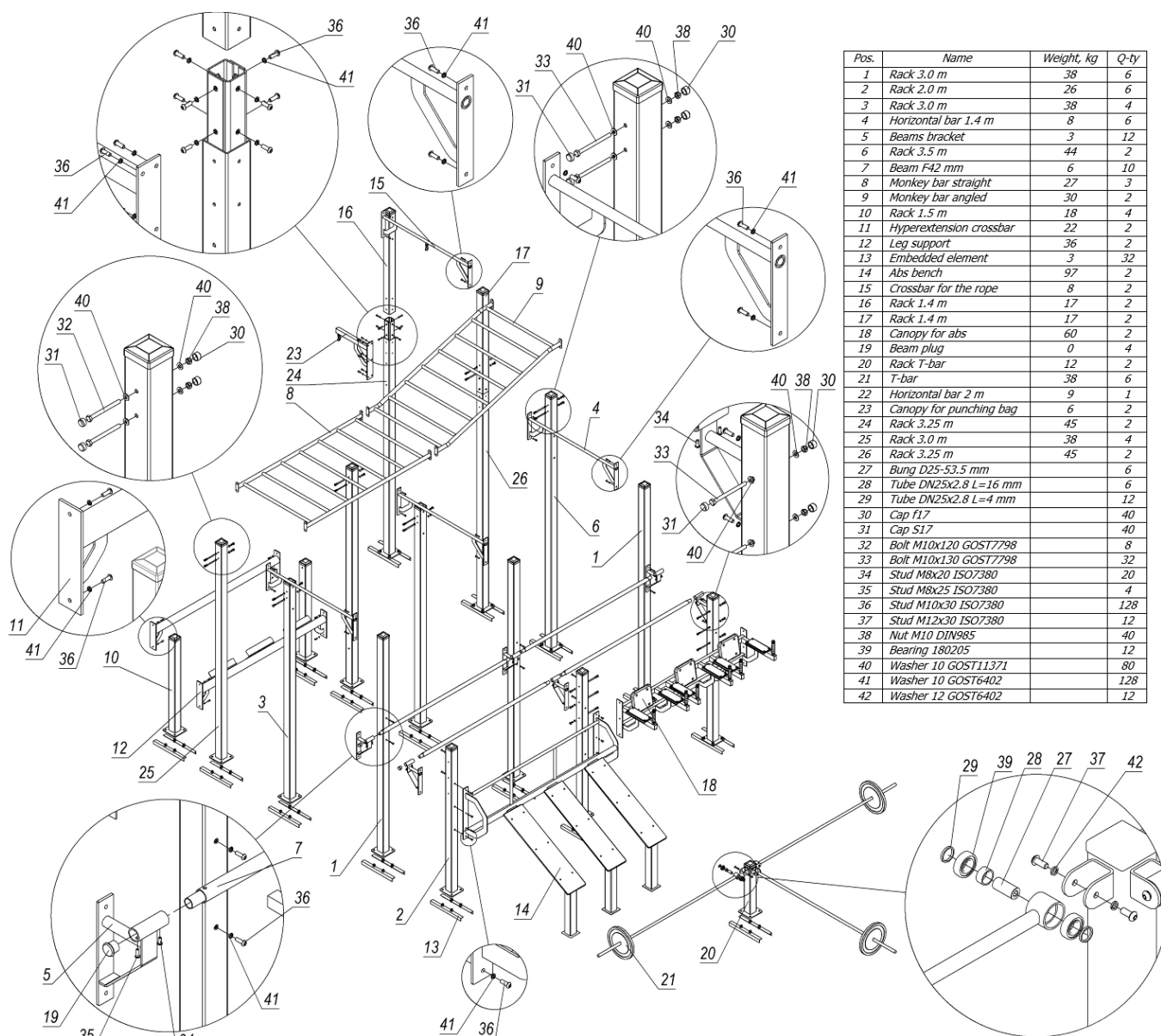
Picture 1 – Components and assembly procedure
