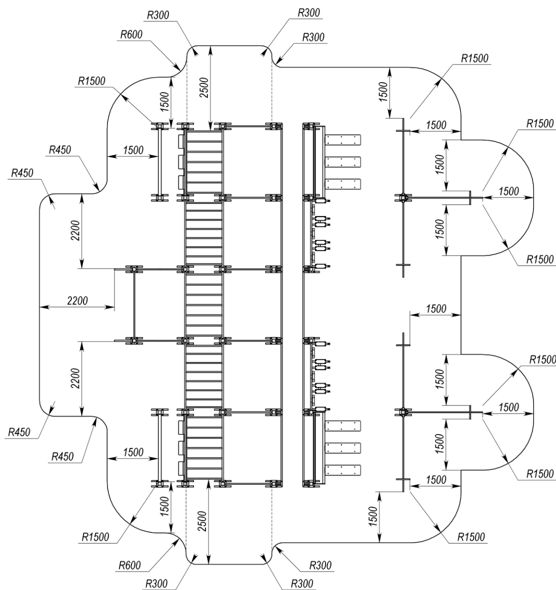
Picture 6 – Safety zone for UT131
