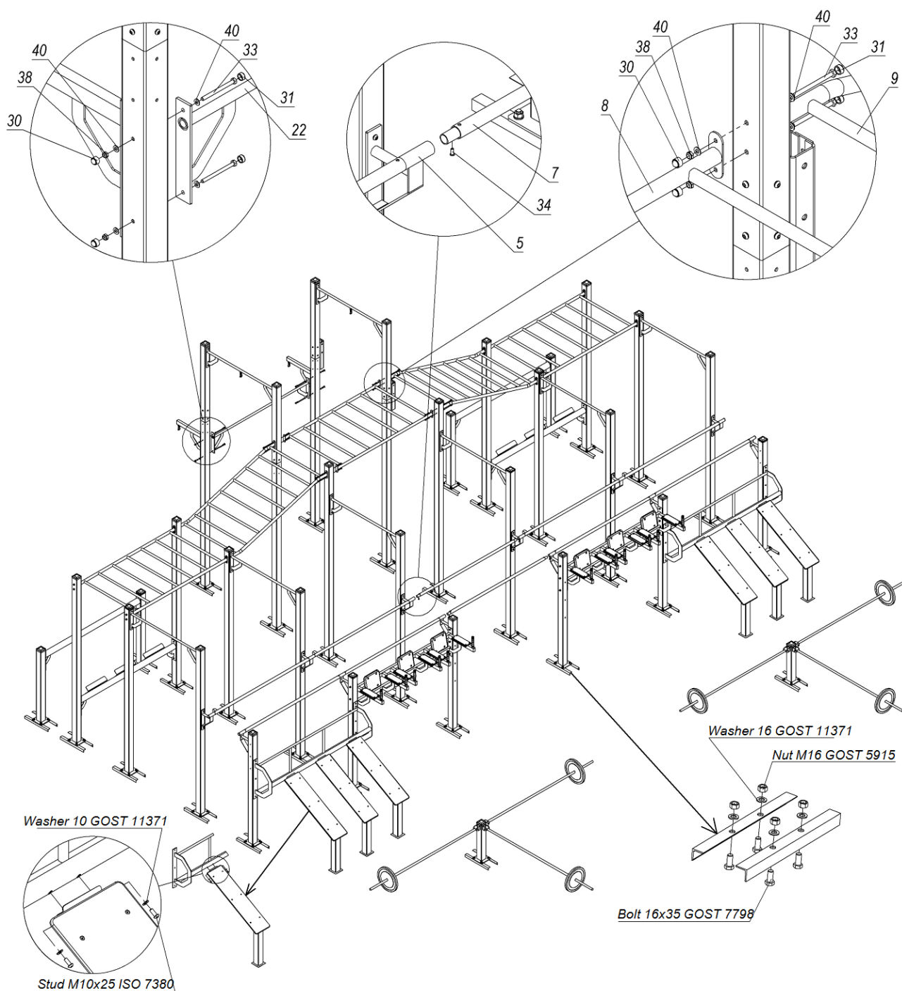
Picture 2 – Components and assembly procedure
