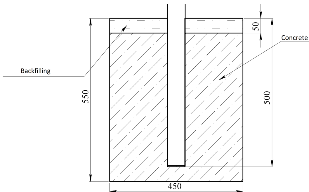
Pic. 3 Scheme of foundation installation
