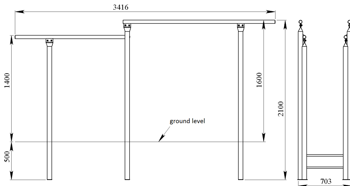
Pic. 2 Overall dimensions
