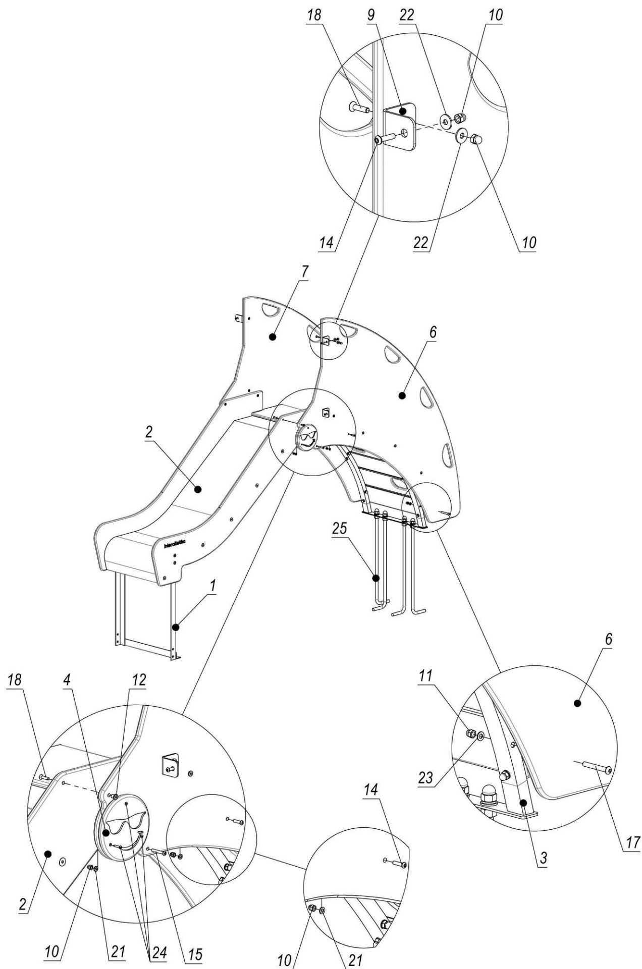
Picture 1.1 – Assembly scheme of slide 0,7m
