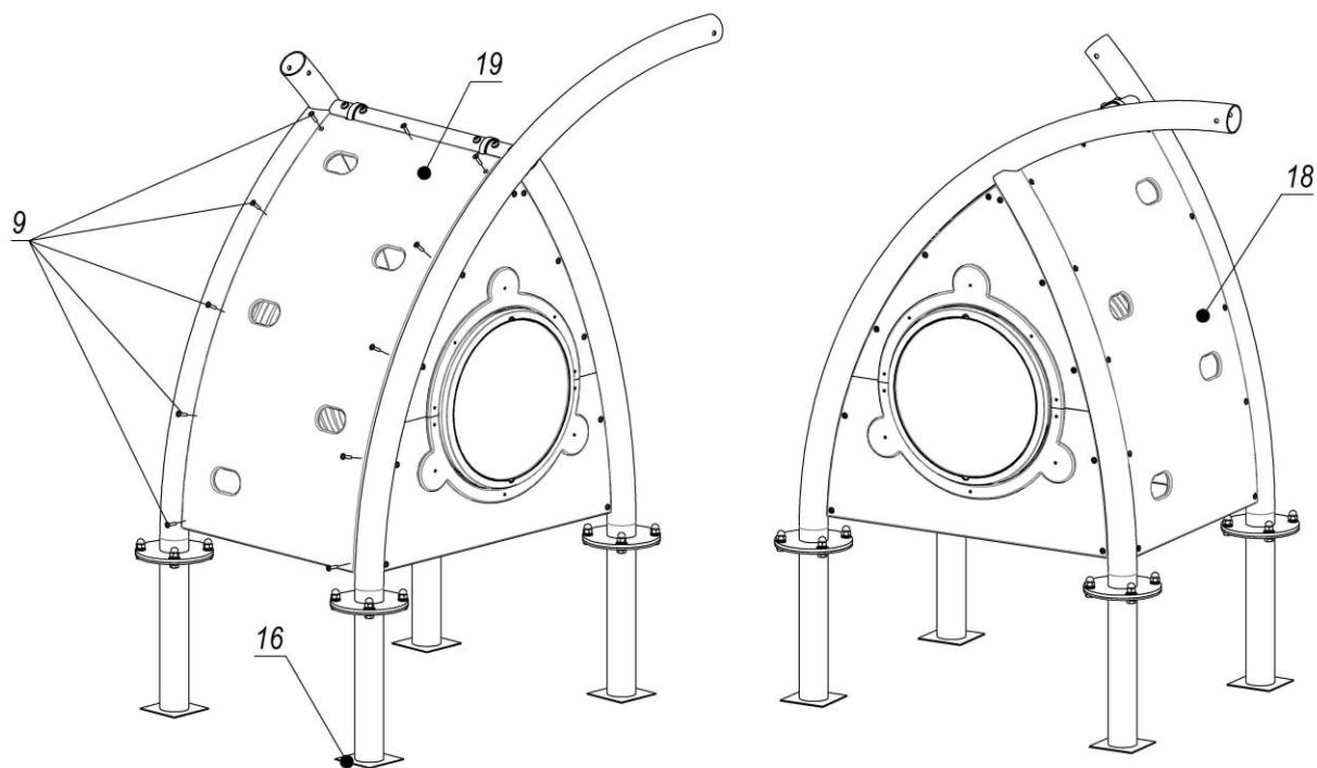
Picture 5 – Installation scheme of climb with adapters (bores in clims with 4/5 adapters pos.18,19, must be bored at the place of installation)
