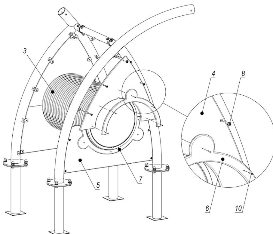
Picture 4 – Tunnel installation scheme
