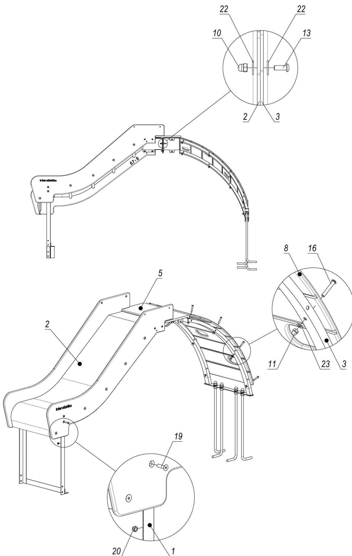
Picture 1 – Assembly scheme of slide 0,7m
