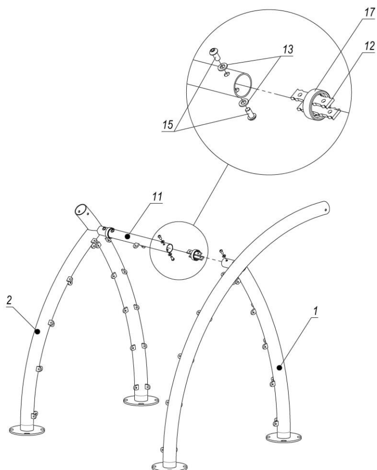
Picture 3 – Rack assembly scheme
